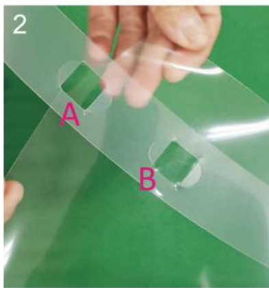
2 Insert and lock left-side Clear Shield tabs into left-side Locking Holes A and B.
